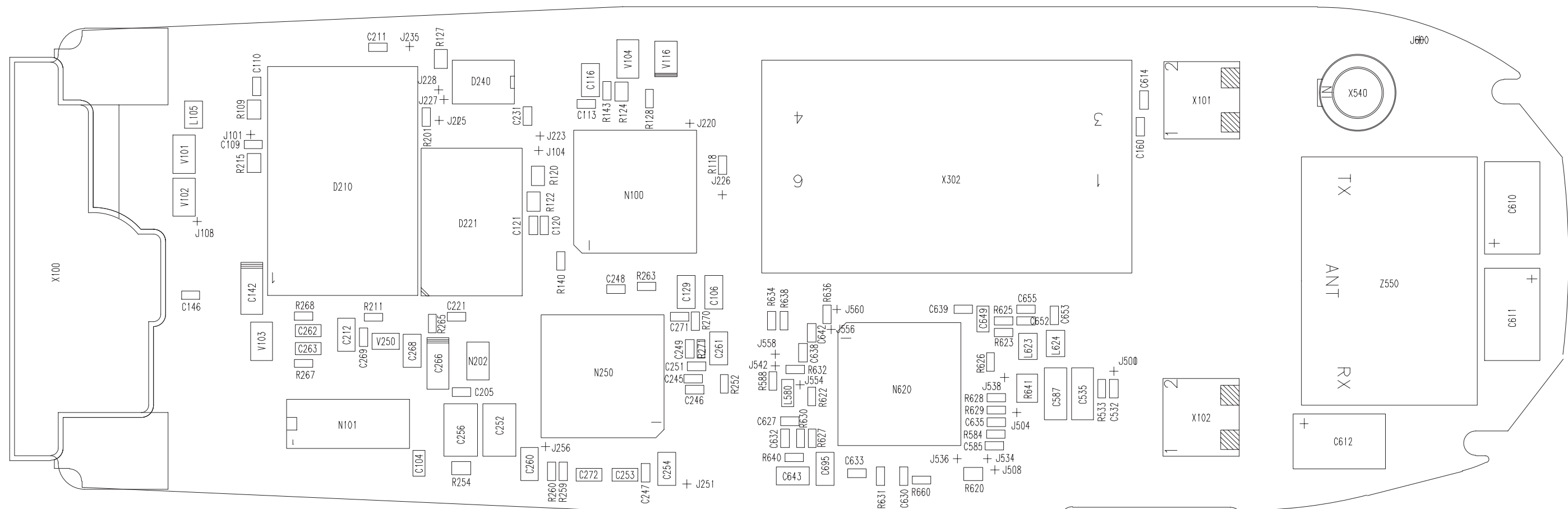
Layout Diagram of UP8S – Bottom (Version 9)
